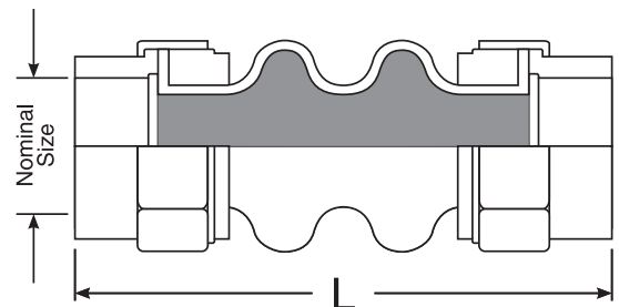
Threaded Union Rubber Expansion Joint
