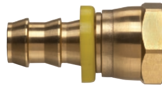
Female Pipe Swivel (NPTF Threads)
